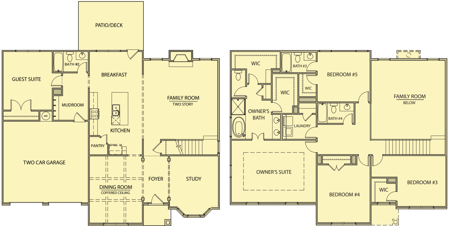
First Floor
