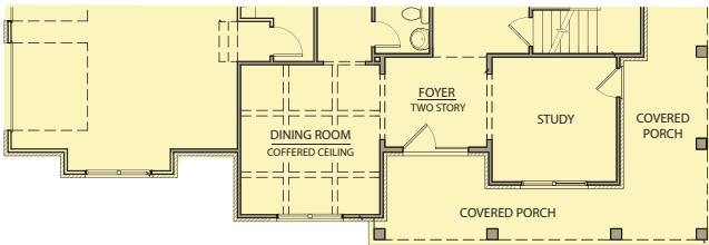
First Floor - Elevation BB
