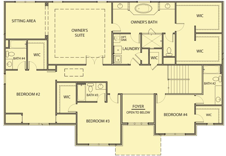
Second Floor - Elevation BB
