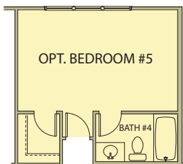
Opt. Bedroom #5/Bath #4 Plan
