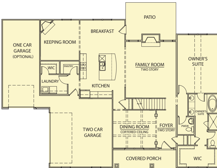
First Floor w/ Keeping Room
